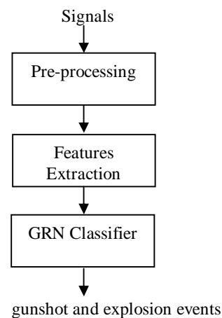
Figure 2. System Architecture of the proposed system
