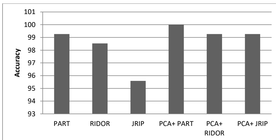
Figure 1. Visualize results for accuracy of different classifiers
