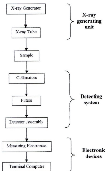
Figure 2. Flow diagram of a sequential EDXRF Analysis
