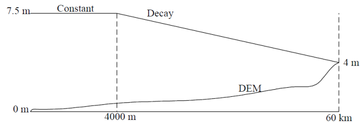
Figure 2: Illustration of 7.5 m Surge Height Decay in Land
