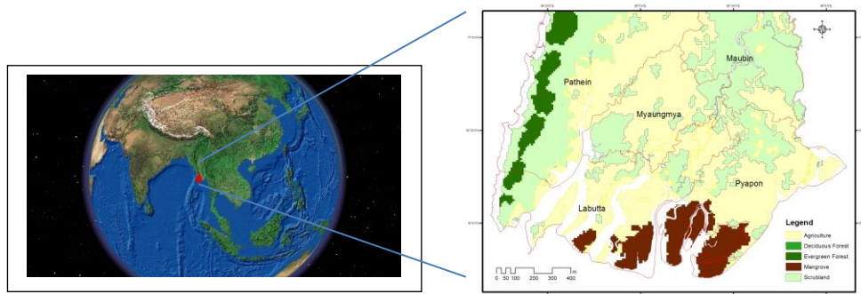
Figure 1: Location and Land cover map of Delta region
