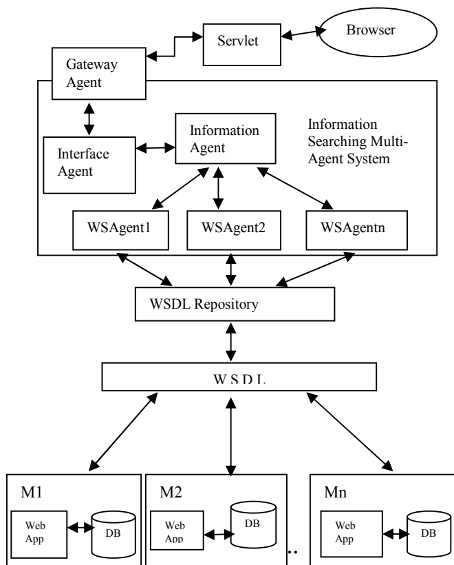
Fig. 1. Medical Information Searching Multi-Agent System Architecture
