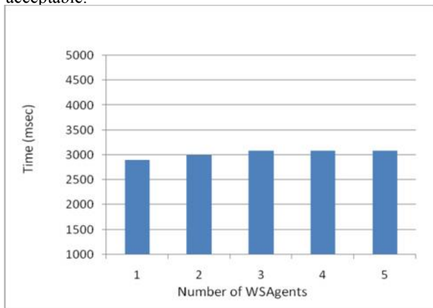
Fig.3 Comparison for Average Processing Time on increasing WSAgents
