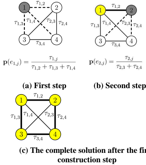
Figure 2: Example of the solution construction for a TSP problem consisting of 4 cities (modelled by a graph with 4 nodes). The solution construction starts by randomly choosing a start node for the ant; in this case node 1. Figures (a) and (b) show the choices of the first, respectively the second, construction step. Note that in both cases the current node of the ant is marked by dark gray color, and the already visited nodes are marked by light gray color (respectively yellow color). The choices of the ant (i.e., the edges) are marked by dashed lines. The probabilities for the different
