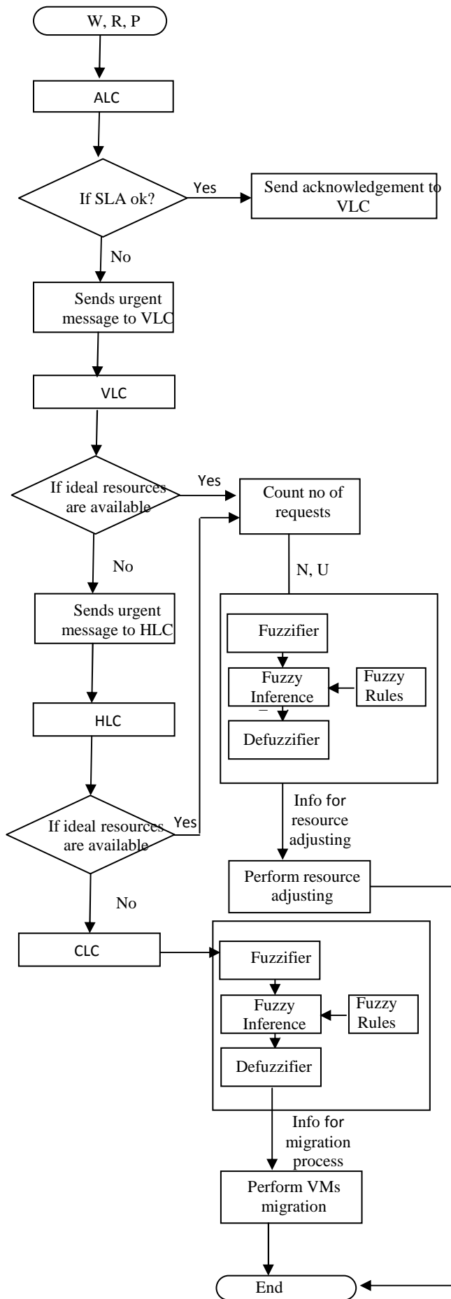
Figure 1. System flowchart of four-level controllers
