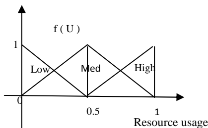
Figure 4. Membership functions of resource usage f(U)
