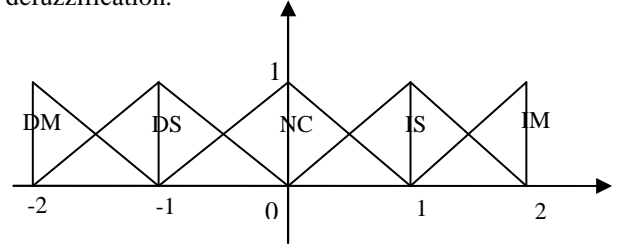
Figure 5. Membership functions of change of resource \Delta V
