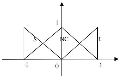
Figure 8. Membership functions of output fuzzy sets
