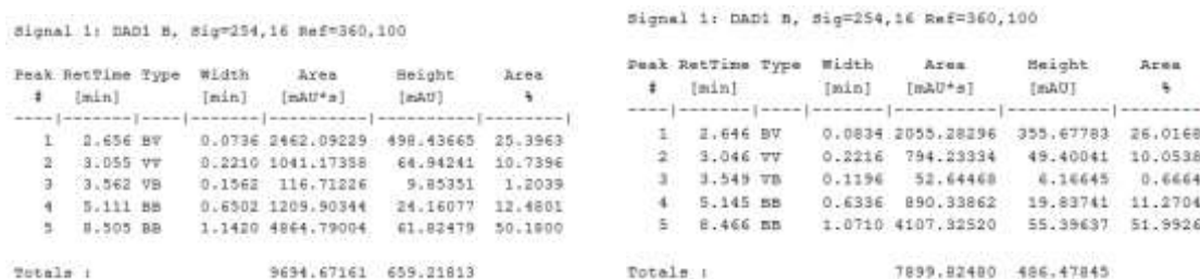
Figure (6) HPLC Chromatogram of Sample A&B
