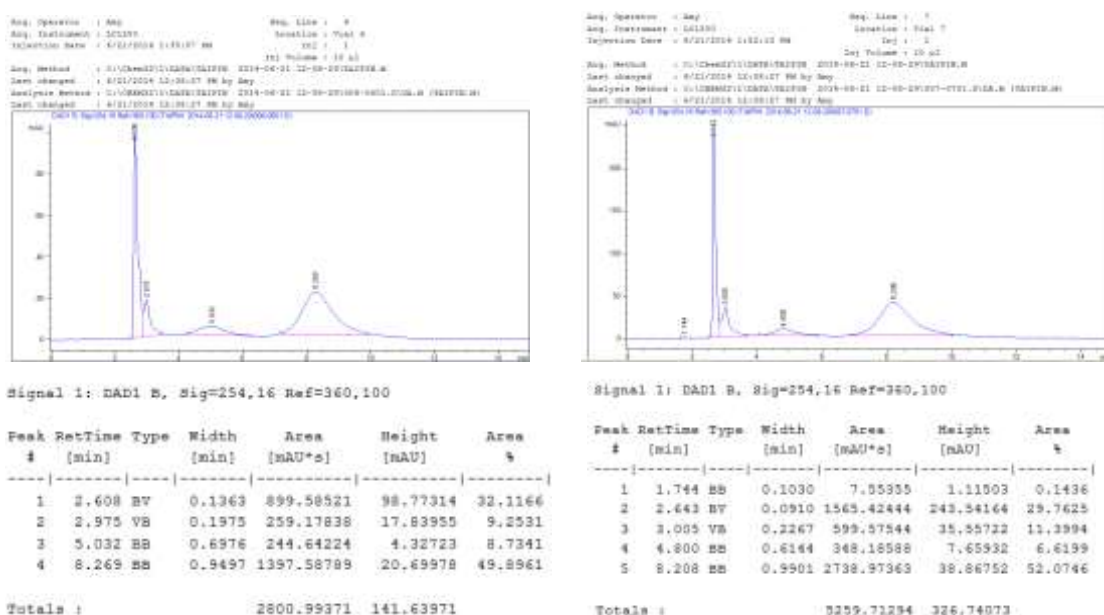
Figure (8) HPLC Chromatogram of Sample E&F
