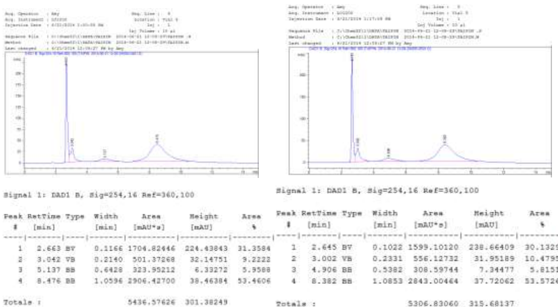
Figure (7) HPLC Chromatogram of Sample C&D
