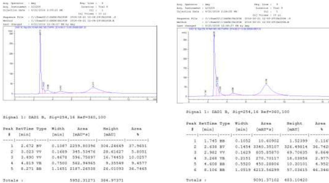
Figure (9) HPLC Chromatogram of Sample G&H
