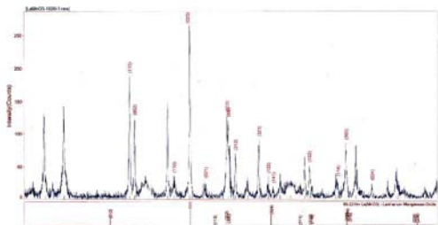
Figure 4. XRD patterns of \text{LaMnO}_3 nanopowder at 1000^\circ\text{C}
