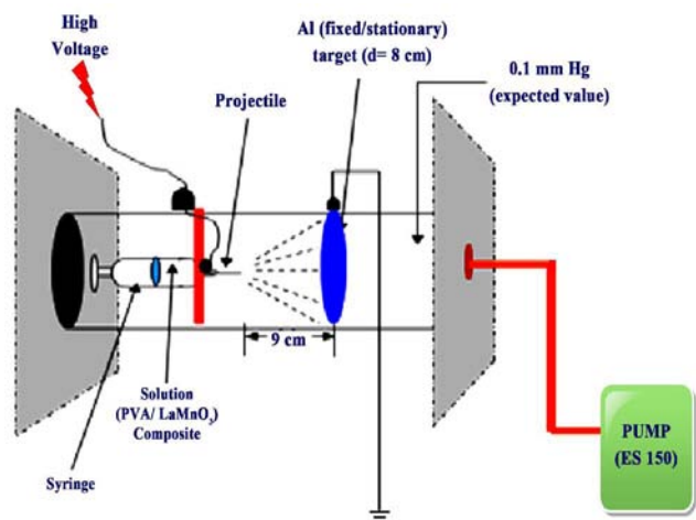
Figure 2. Schematic diagram of electrospinning set-up
