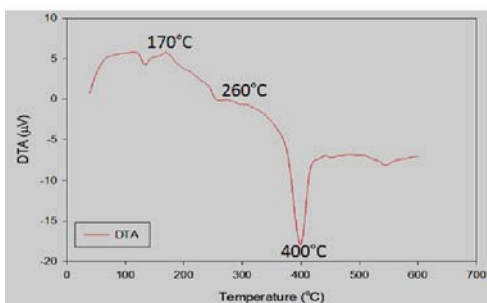
Figure 3 (a) DTA analysis of \text{LaMnO}_3 nanopowder
