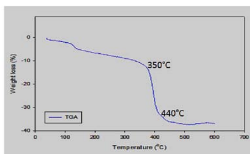
Figure 3 (b) TGA analysis of \text{LaMnO}_3 nanopowder
