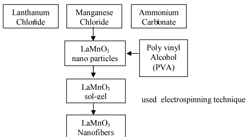
Figure 1. Flowchart of preparation of \text{LaMnO}_3 Nanofibers.
