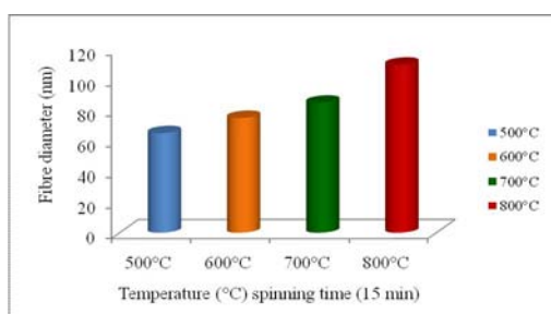
Figure 6. Temperature dependence of LaMnO 3 nanofibers
