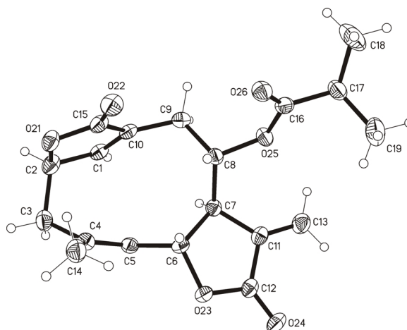
Fig. 1. Crystal structure of 17,19-dihydrodeoxyelephantopin ( 2 ) showing 50% thermal ellipsoids. The bonds between carbon and hydrogen are shown as thin lines. Both C18 and C19 are saturated carbon atoms in contrast to the previous structure 1 where C19 was an unsaturated carbon.
